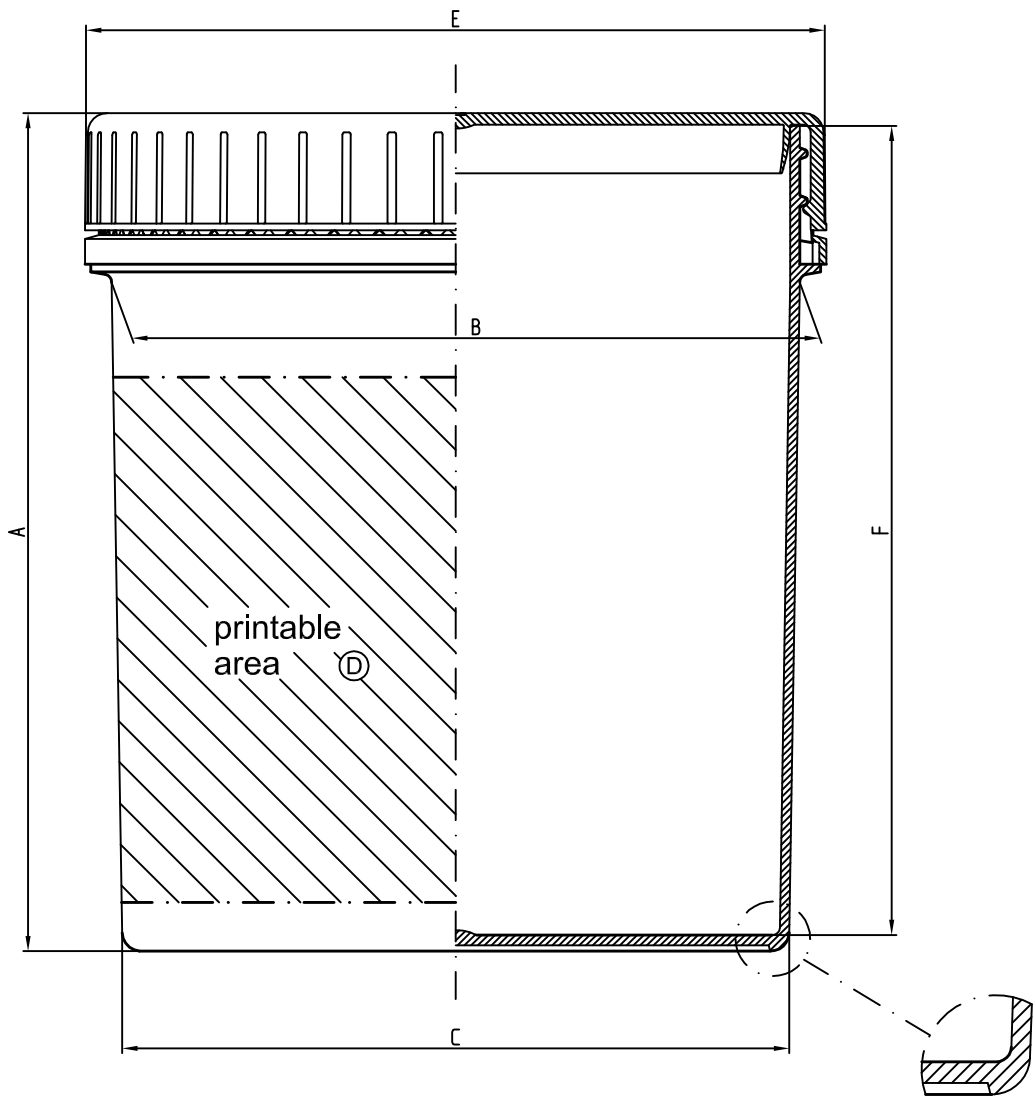
Screw-top container Ø71 - 315 R1 PP with Tamper-evident Closure
